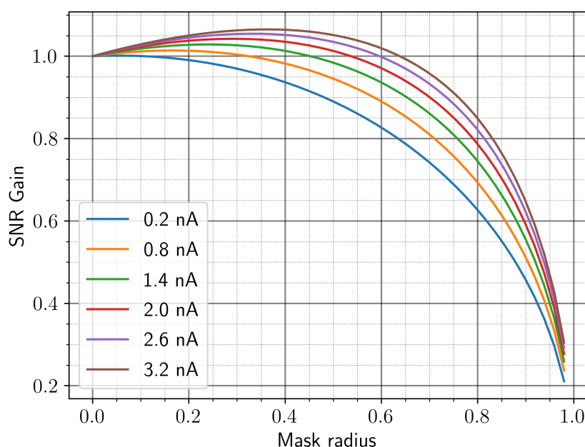
Figure 9. The SNR gain as function of mask radius for different incoming currents. The SNR gain is defined as the ratio of the SNR with the SNR when the mask radius is zero.
