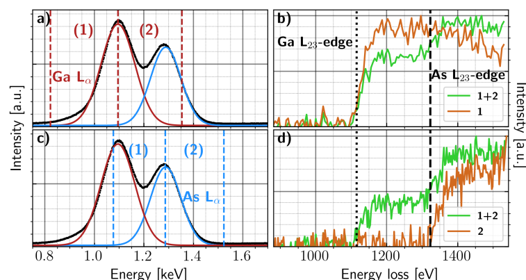
Figure 4. (a) The EDX spectrum of GaAs where the Ga peak is fitted with a Gaussian to indicate the extent of the X-rays originating from the de-excitation of the Ga atom. The red and blue line indicate the extent of the X-ray lines in the energy spectrum. (b) The background-subtracted EEL spectra using the X-rays in the regions are indicated by the legend. When only using X-rays from region 1 , it is seen that only the Ga L_{23} edge is selected without the As L_{23} edge (brown). When regions 1+2 are selected, electrons from both edges are seen (green). (c) The same as (a) where the X-ray regions, out which the coincidence events are chosen, have been modified. (d) The background-free EEL spectrum where, by selecting the proper X-ray window ( region 2 ), only the As L_{23} edge is selected (brown). When regions 1+2 are selected, electrons from both edges are seen (green).
